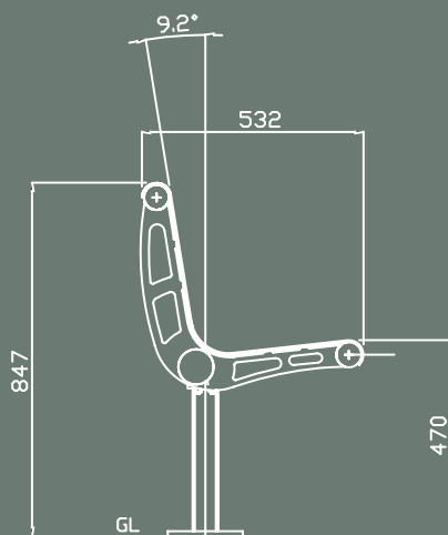
TYPICAL ELEVATION
