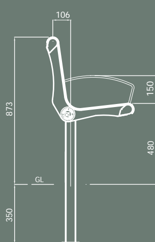
SPIGOT MOUNTED TYPE TYPICAL ELEVATION WITH MANNHEIM ARM
