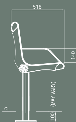
SUB-SURFACE MOUNTED TYPE TYPICAL ELEVATION WITH FLORENTINE ARM
