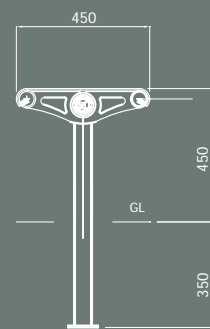
SPIGOT MOUNTED TYPE TYPICAL ELEVATION
