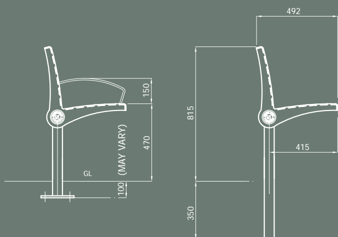
SPIGOT MOUNTED TYPE TYPICAL ELEVATION
