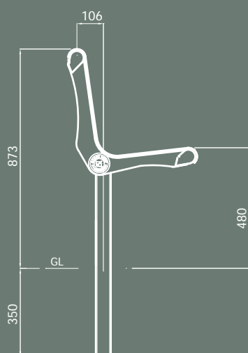
SPIGOT MOUNTED TYPE TYPICAL ELEVATION
