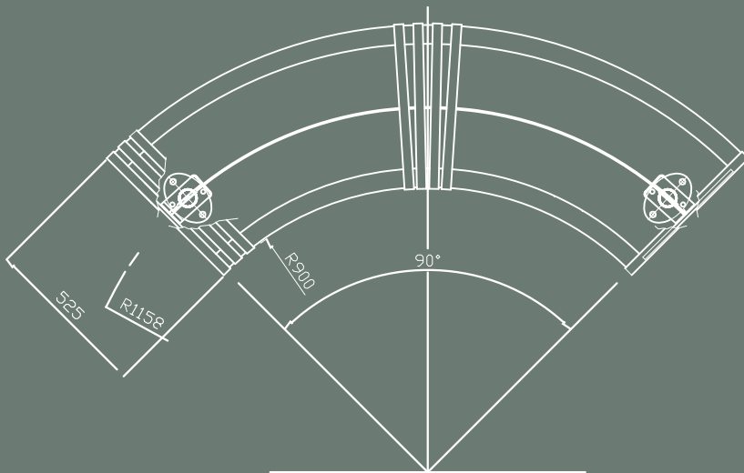
PLAN - SOME STRAPS REMOVED FOR CLARITY
