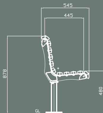
TYPICAL ELEVATION
