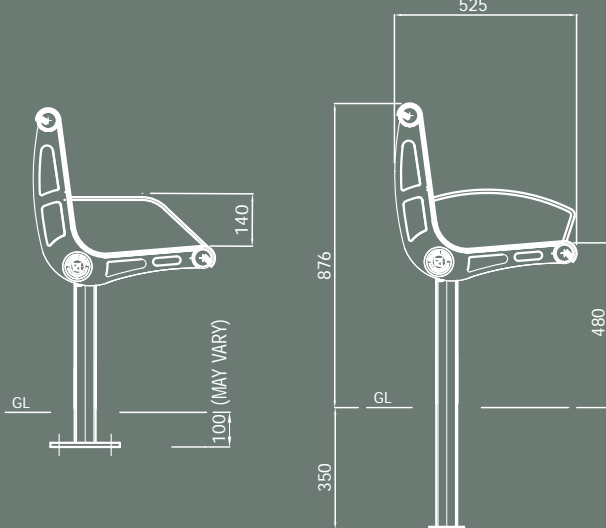
SUB-SURFACE MOUNTED TYPE TYPICAL ELEVATION WITH FLORENTINE ARM
